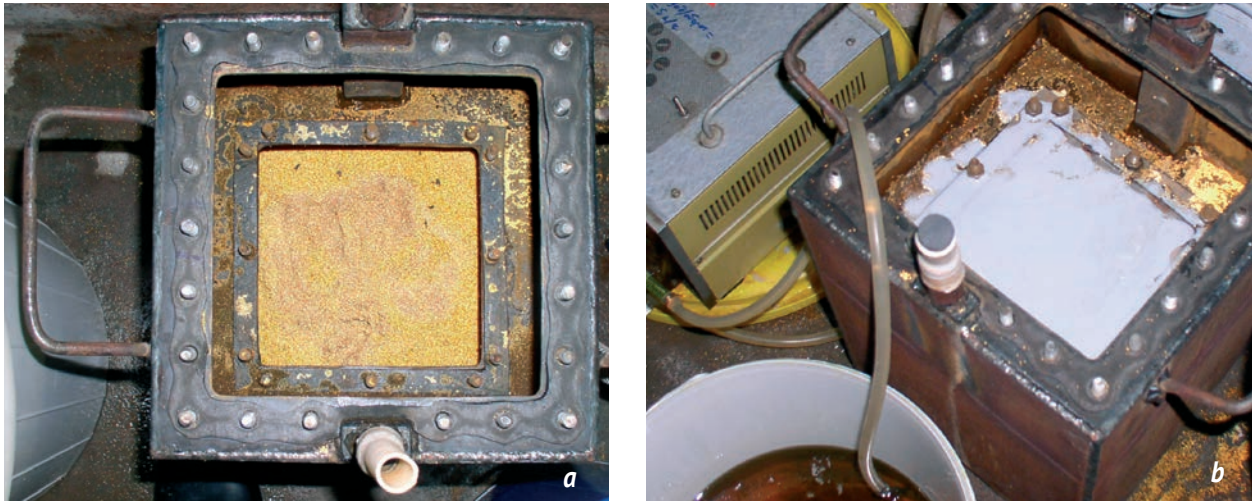
Fig. 1. IER conditioning in the container: a – dewatering, b – embedding in a polymer binder
