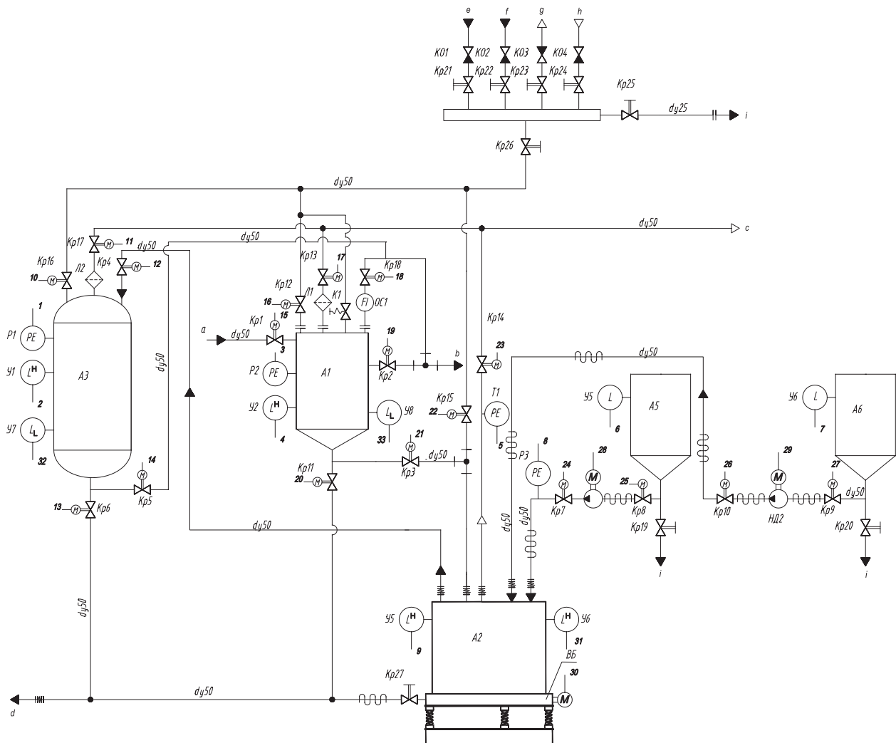
A1 – batcher, A2 – container, A3 – montejus, A5 – vessel for epoxy resin, A6 – vessel for hardener, BB – vibrobench; a , b – IER injection and backflow, c – blowoff, d – special sewage, e – decontamination solution, f – water, g – vacuum, h – compressed air, i – drain
